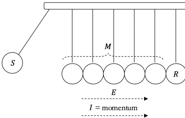
Figure 5 The energy flow diagram schematically describing a process where a metal ball transfers energy to another metal ball, using a number of intermediary metal balls as the material carrier, and momentum as the immaterial carrier.
